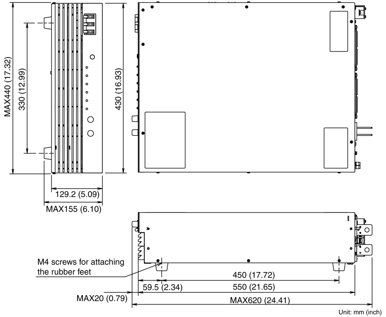
PAT-T Series Outline Drawing
