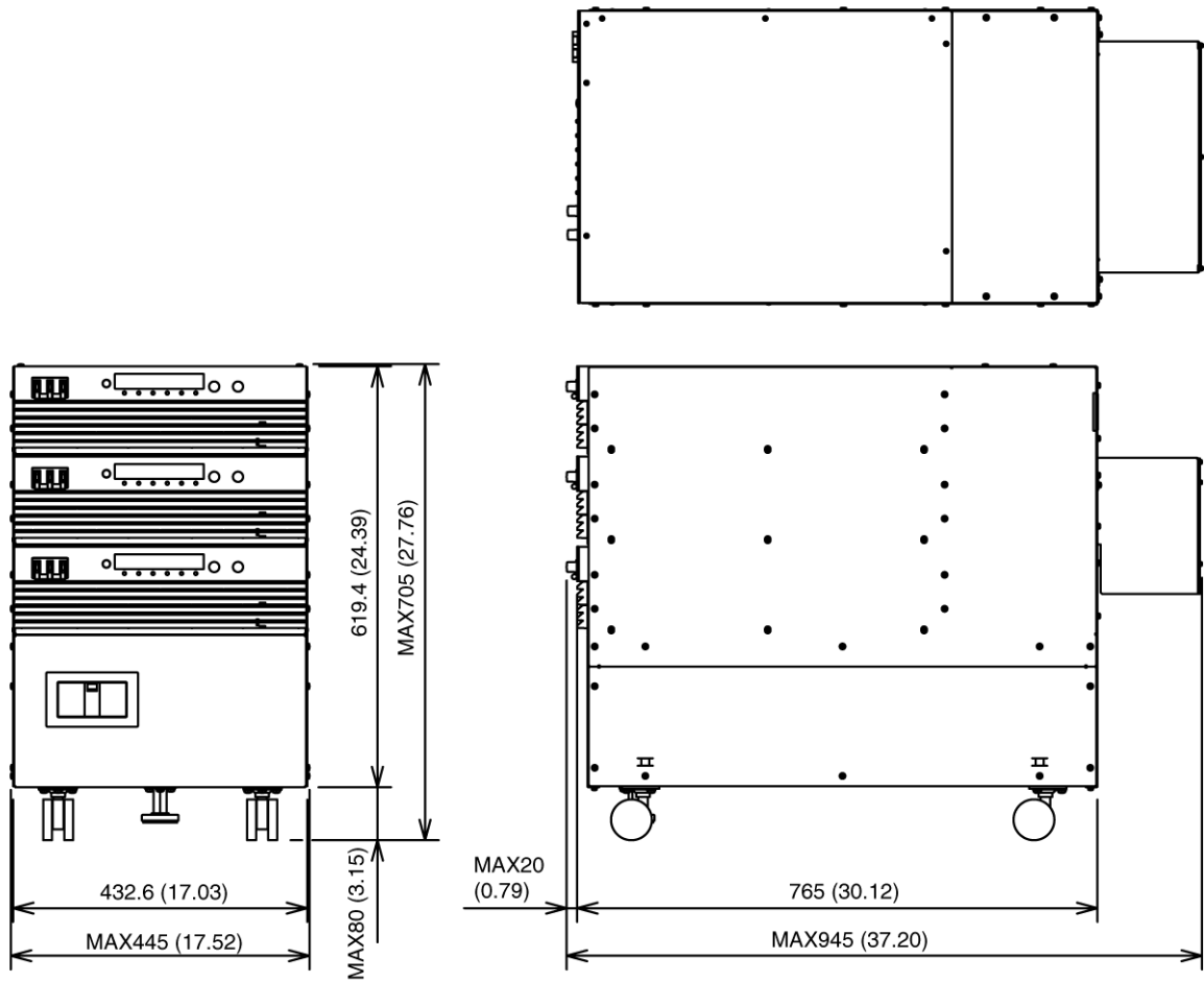
PAT-TMX Series 24 kW System Outline Drawing
