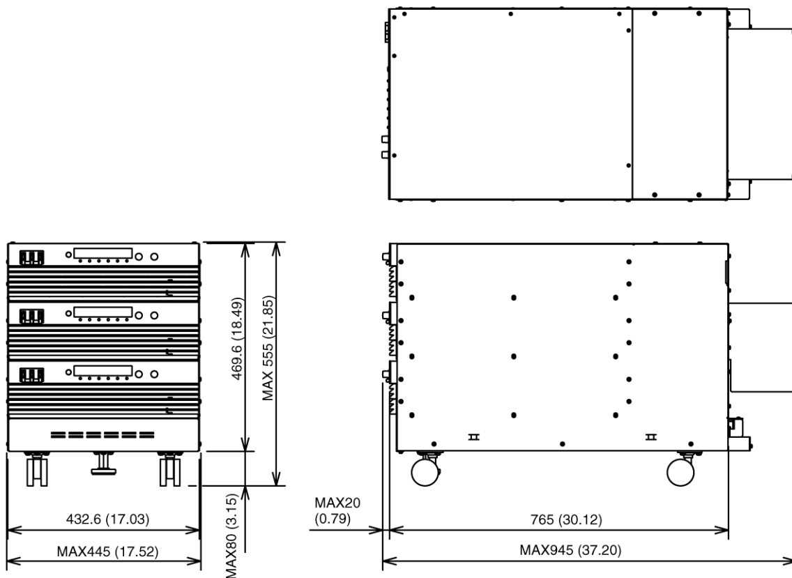
PAT-TM Series 24 kW System Outline Drawing
