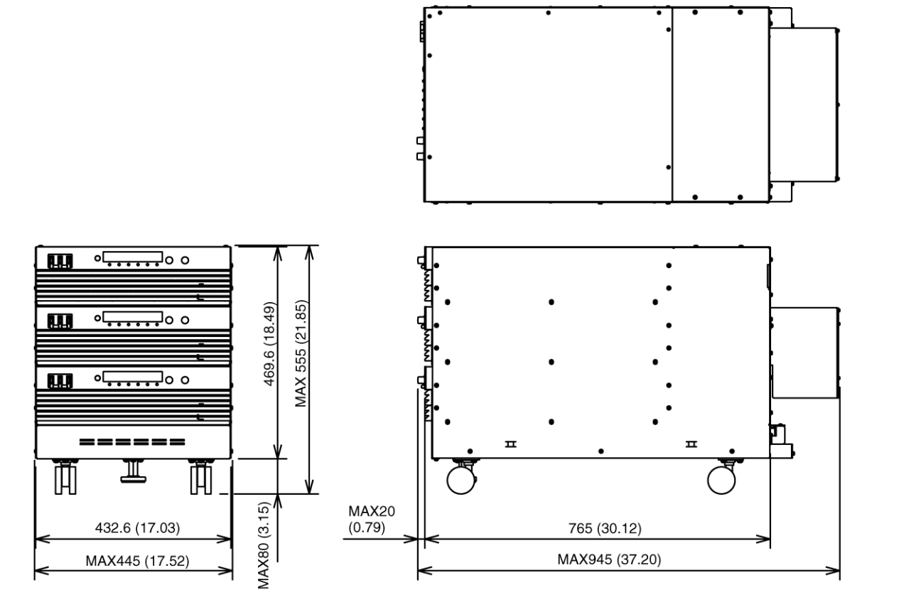
PAT-TM Series 24 kW System Outline Drawing
