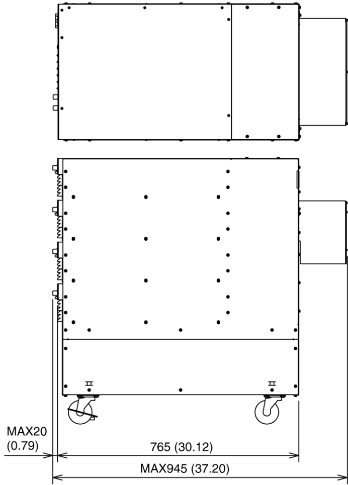
PAT-TMX Series 32 kW System Outline Drawing
