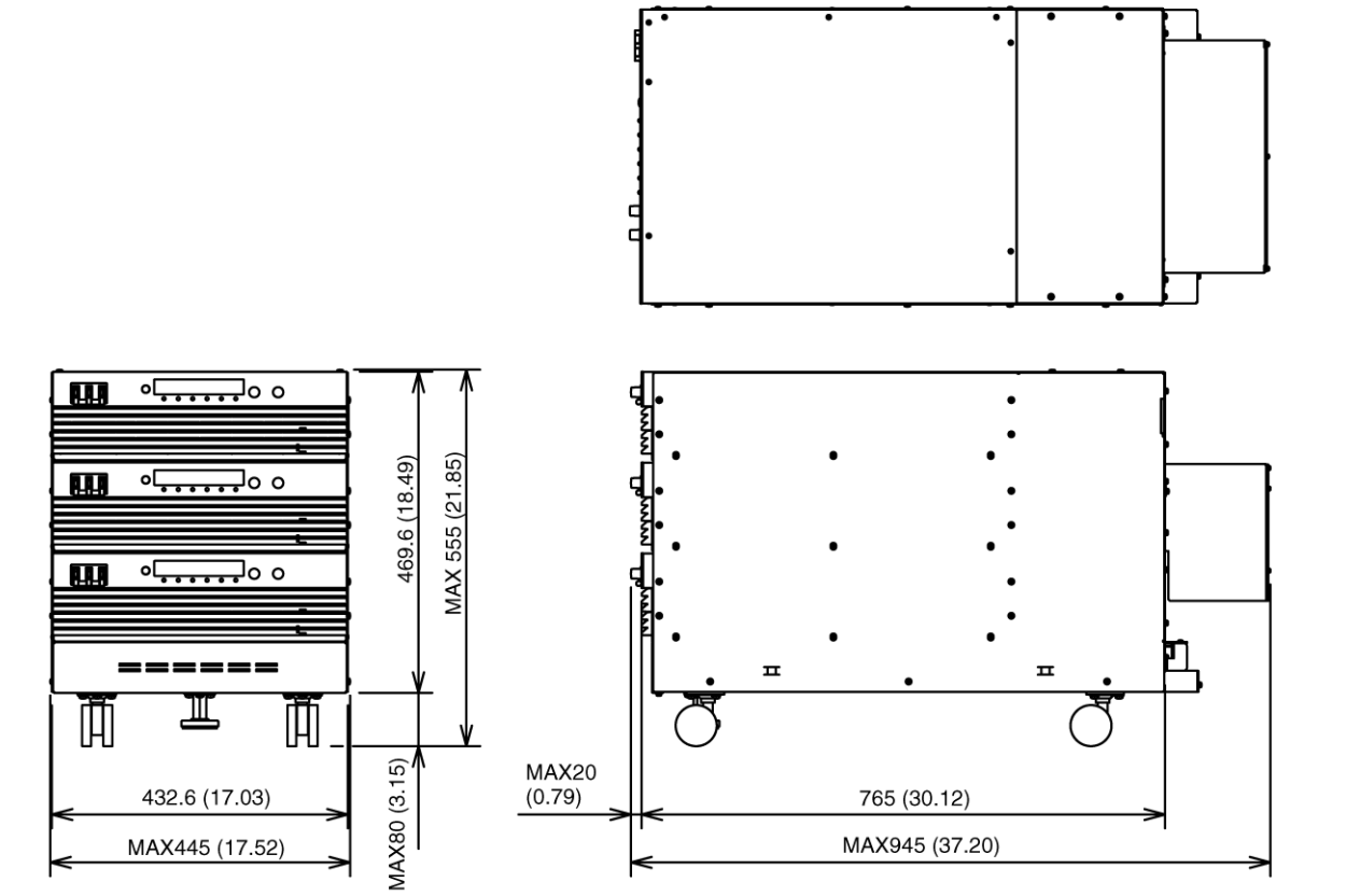
PAT-TM Series 24 kW System Outline Drawing
